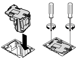
Securing screws
