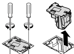
Securing screws
