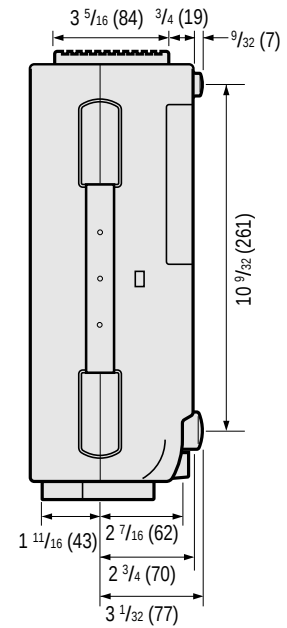
Vista frontal
